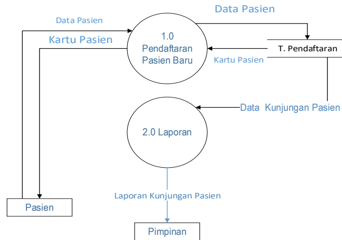
Gambar 4 Data Flow Diagram level 2
